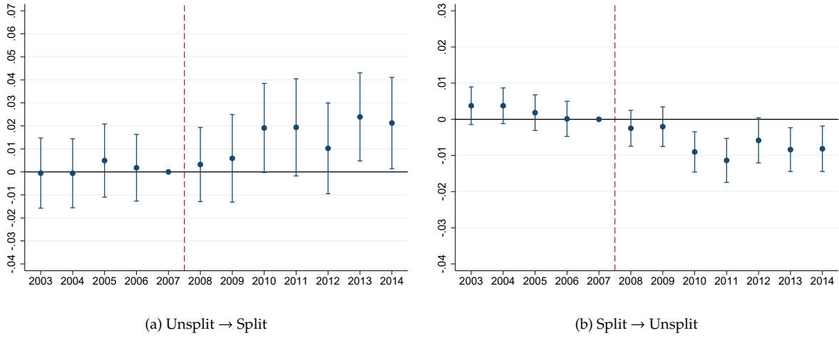
Figure 6: Differences-in-Discontinuity Design
